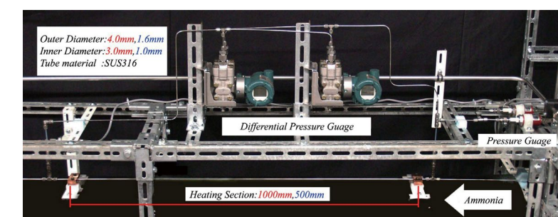
Fig. Test section
