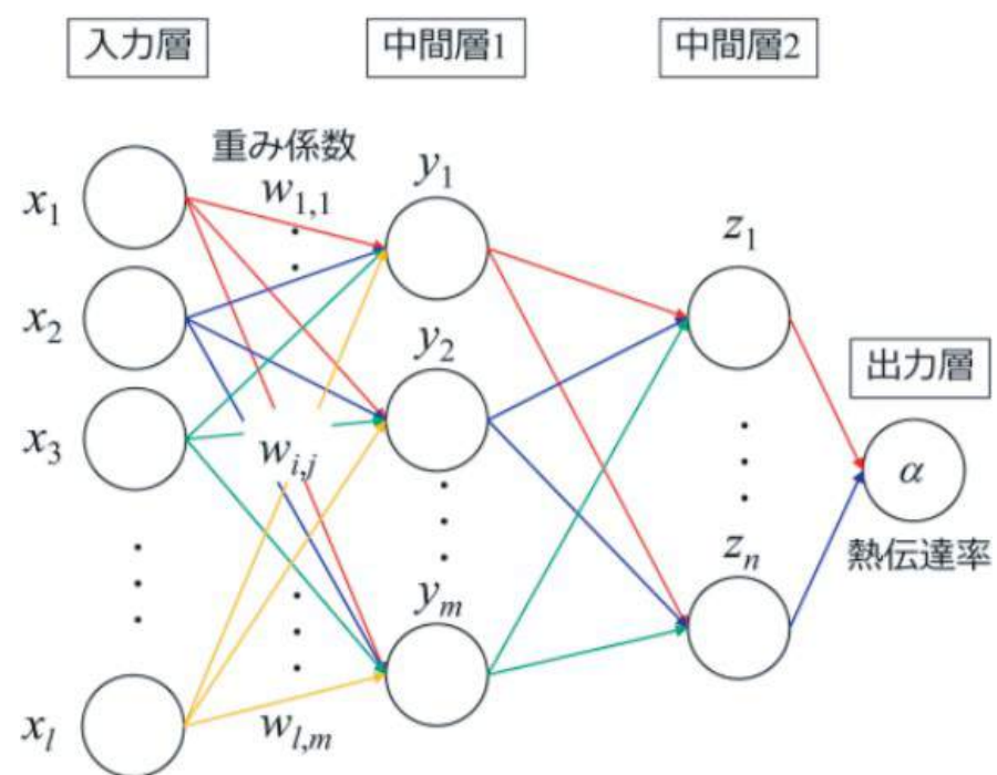
Fig.2 Conceptual diagram of ANN
